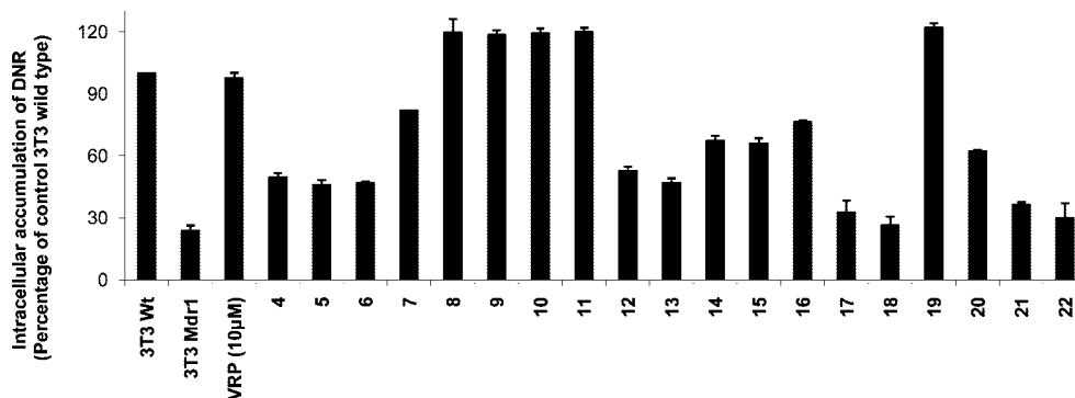
Figure 3. Modulation of daunorubicin accumulation by 10 \mu M bis-pyranobenzoquinone derivatives in NIH-3T3 MDR1 cells. Results are expressed as percentage of daunorubicin uptake in NIH-3T3 MDR1 cells in the presence or absence of compounds with respect to the accumulation in NIH-3T3 Wt cells (100%). 10 \mu M verapamil was used for comparison. The data are the average of three independent experiments \pm SD.
