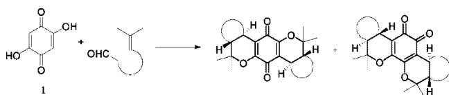
Scheme 2. Bis-pyranobenzoquinones from 1 and Unsaturated Aliphatic Aldehydes
